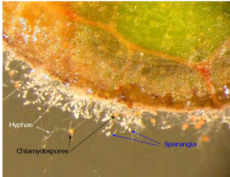
Figure 2. Hyphae, sporangia, and chlamydospores on a leaf disk in laboratory medium. Jennifer Parke, Oregon State University
