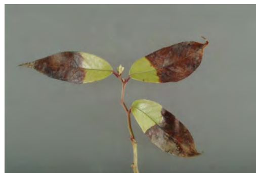
Figure 21. Leaf lesions caused by P. ramorum on leucothoe. Central Science Laboratory, DEFRA (UK) (Crown Copyright)
