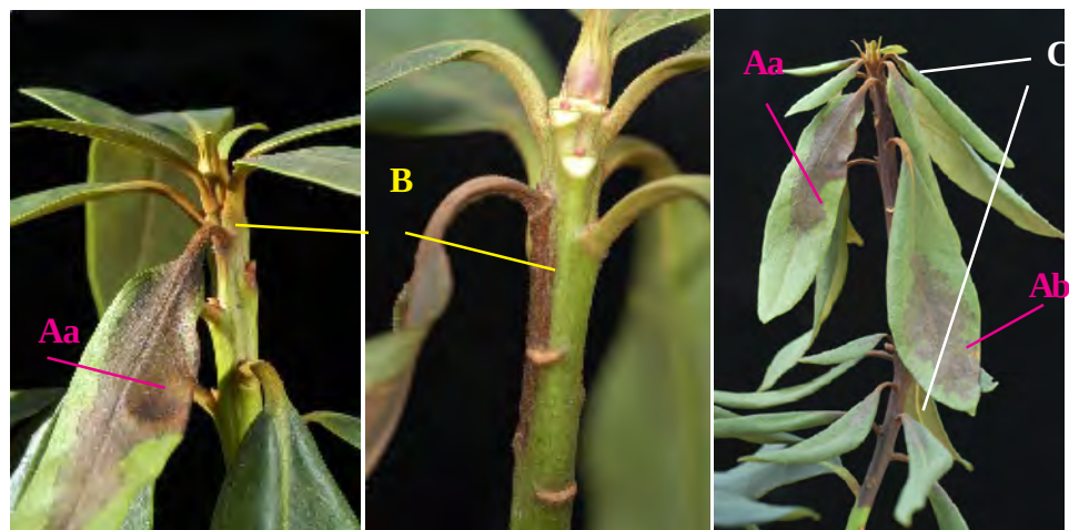
Figure 5. Symptom progression (approximately 3 weeks) of a laboratory infected R. 'Cunningham's White' . (Aa & Ab) indicate initial leaf infection sites. Infection Aa develops through petiole, forming stem canker (B). Infection develops upward and downward in stem, and into leaf petioles and bases of leaves (C). Steve Tjosvold, UC Cooperative Extension
